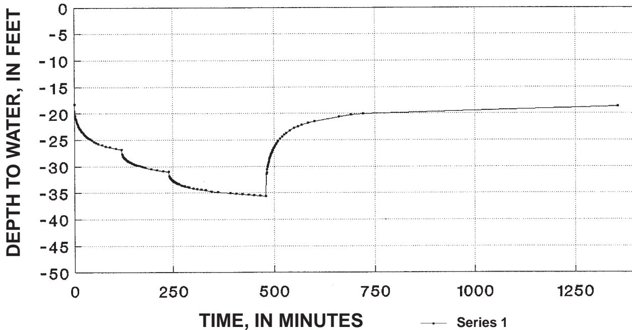
Figure 2: Plot showing depth to water during aquifer test on well #4. Pumping rates are 300, 400, and 500 gallons per minute.
