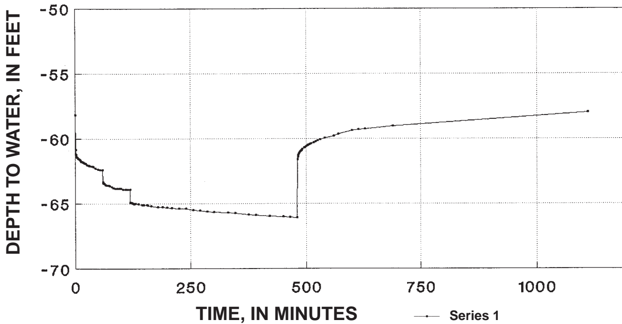
Figure 3: Plot showing depth to water during aquifer test on well #6. Pumping rates are 500, 600, and 690 gallons per minute.
